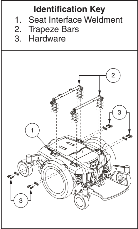
Figure 10. Seat Height/Angle Adjustment
