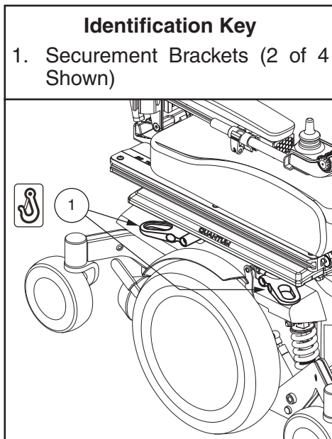
Figure 9. Transit System Securement Brackets
