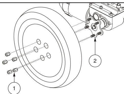
Figure 17. Q6 Edge 2.0 Drive Wheel
