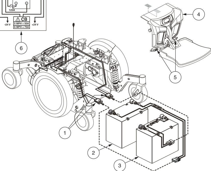
Figure 19. Battery Installation
