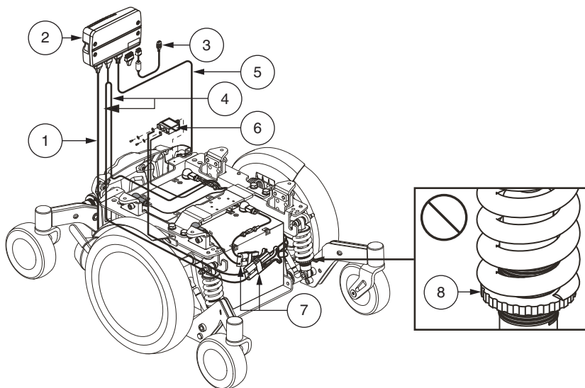
Figure 1. Q6 Edge 2.0 Electrical Components
