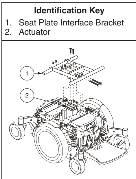
Figure 8. Power Elevating Seat Actuator
