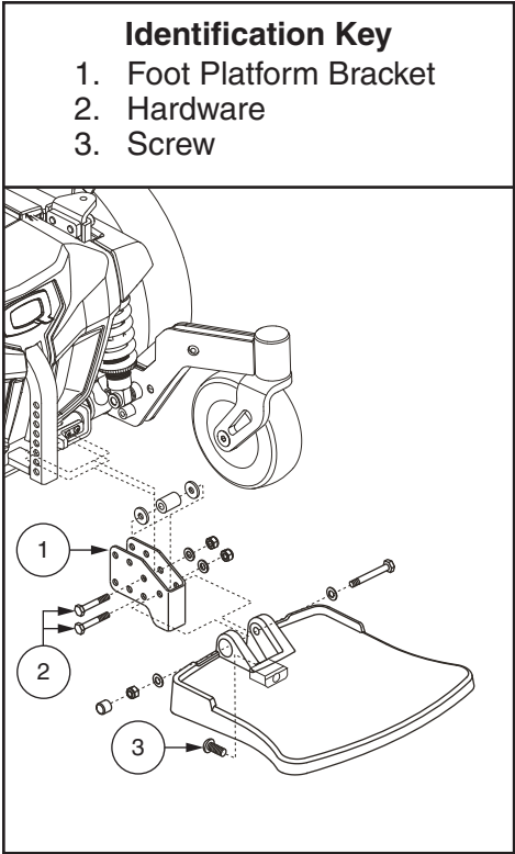
Figure 13. Foot Platform Adjustment
