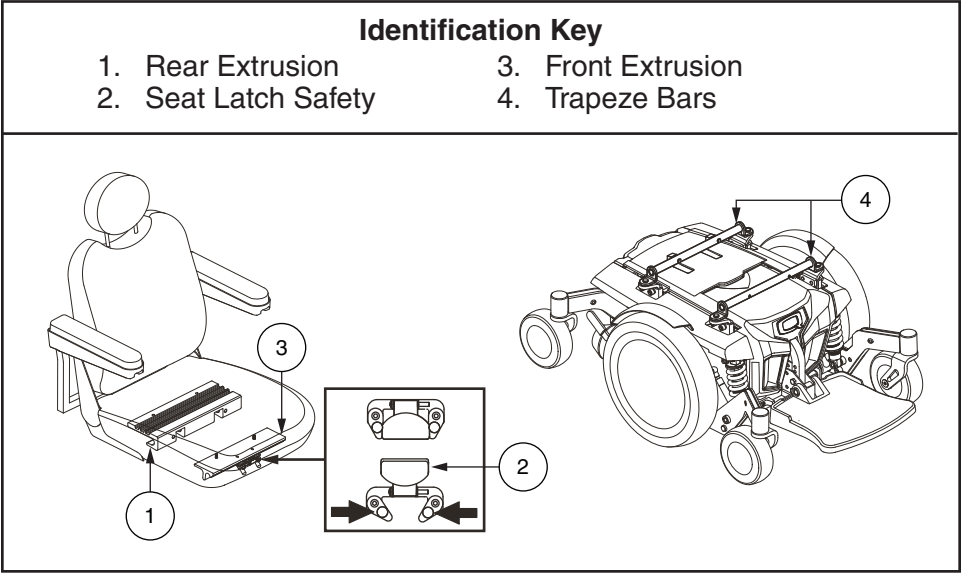
Figure 5. Universal Mounting System and Contour Seat
