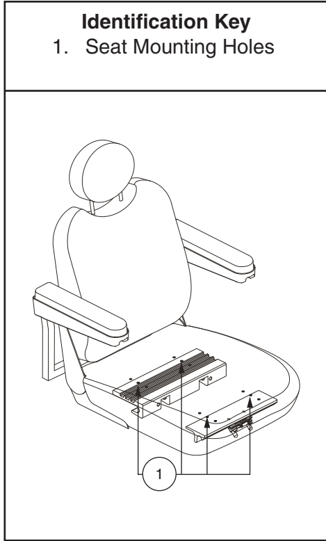
Figure 11. Seat Position Adjustment
